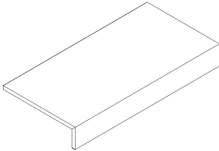
MITRED L SHAPE 45° WITH DRIPSTONE
